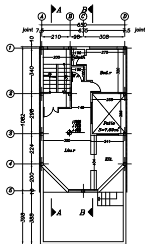
TYPICAL FLOOR PLAN SC. 1:100
