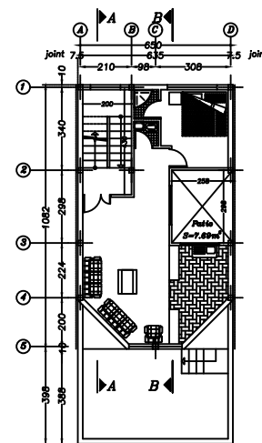
DECORATION PLAN SC. 1:100
