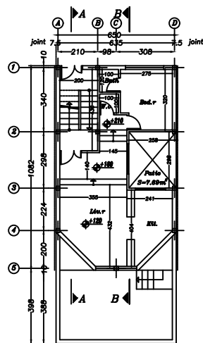
GROUND FLOOR PLAN SC. 1:100
