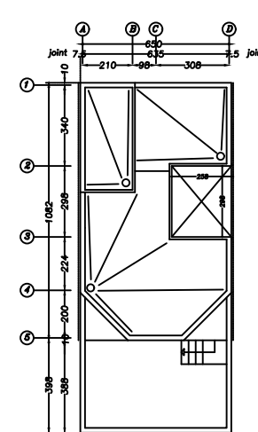
ROOF PLAN SC. 1:100
