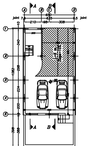
BASEMENT PLAN SC. 1:100
