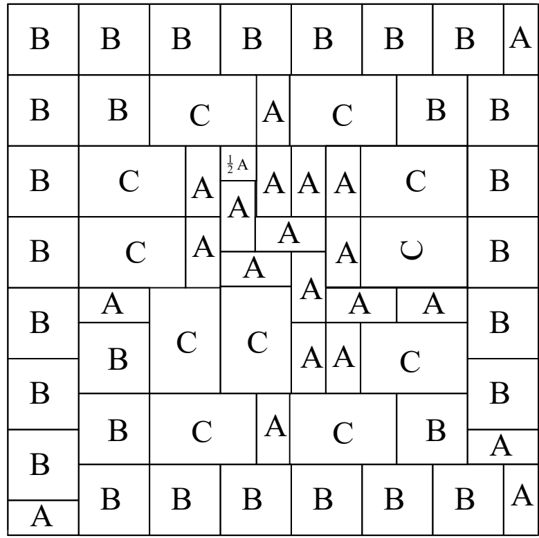
PATIO PAVER PLAN Area : 65.34 sq. ft.
